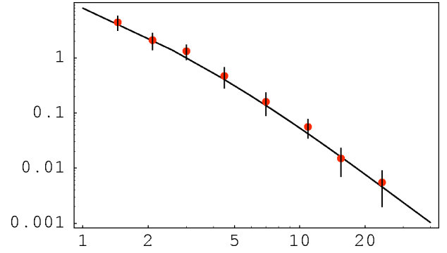
FIG. 3. Cross-section d\sigma_{ee \rightarrow ee\rho^0\rho^0}/dQ^2 [pb/GeV ^2 ] as a function of Q^2 . The theoretical cross section is plotted for the best fitted parameters which are C_1 = 1.2 \text{ GeV}^2 , \langle W_1 \rangle = 3.0 \text{ GeV} and \langle W_2 \rangle = 1.5 \text{ GeV} .
