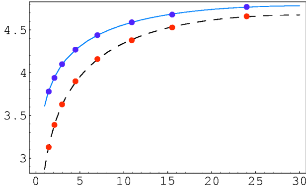
FIG. 2. The muonic parameters \langle W_{1,(\mu)} \rangle^2 (solid) and \langle W_{2,(\mu)} \rangle^2 (dashed) as functions of Q^2 .
